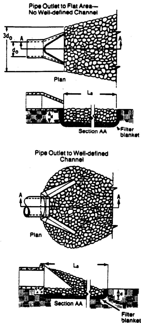
FIGURE 3.22 TYPICAL DETAILS FOR ROCK OUTLET PROTECTION (Modified from State of North Carolina, 1988)
